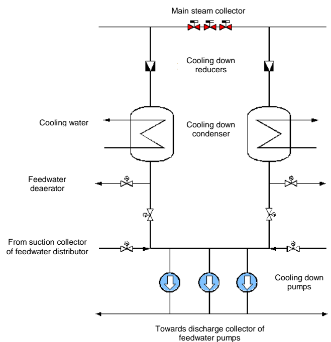
Figure 1-10: Cool-down system
